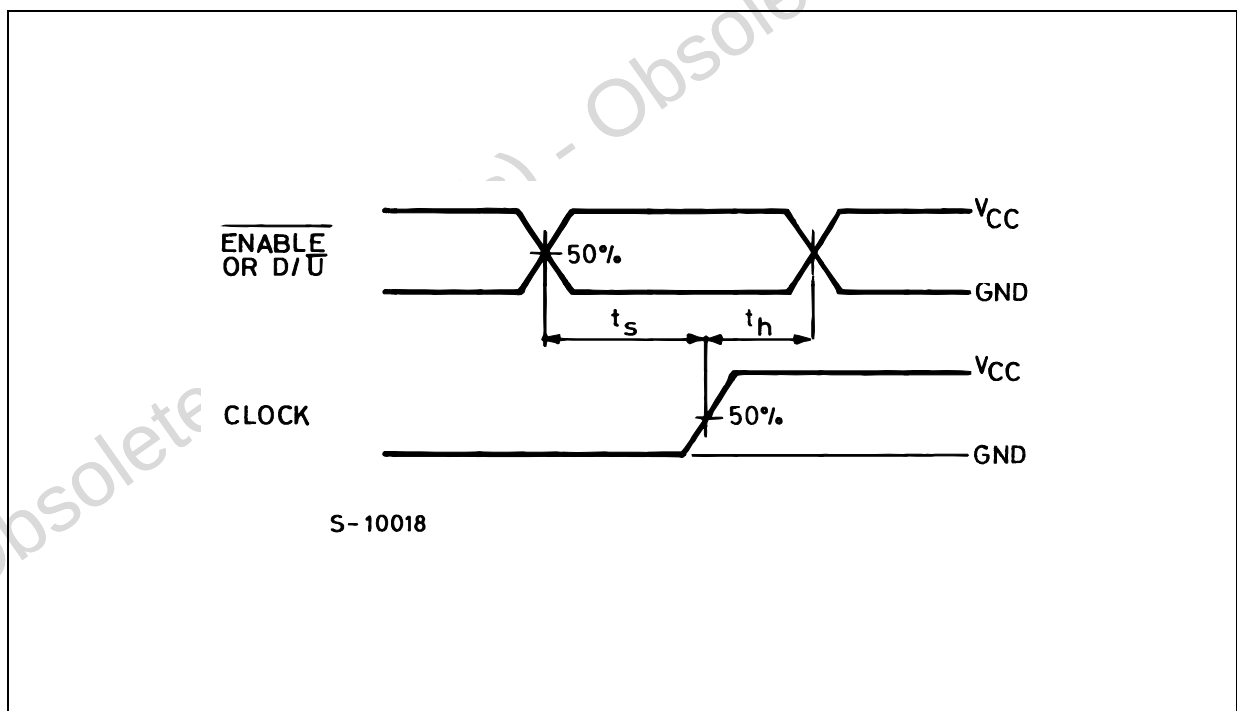
WAVEFORM 6 : SETUP AND HOLD TIME ( f=1\text{MHz} ; 50% duty cycle)
